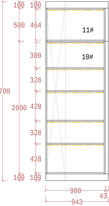
INNER VIEW C
