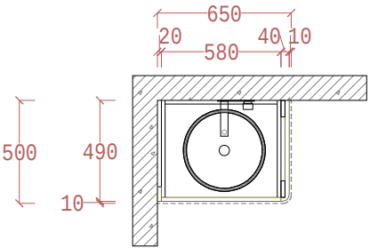
PLAN VIEW floor
