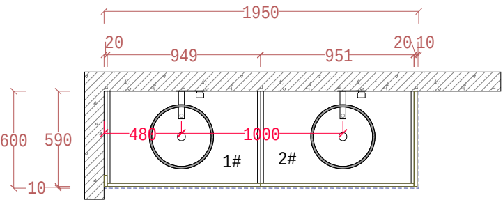
PLAN VIEW floor
